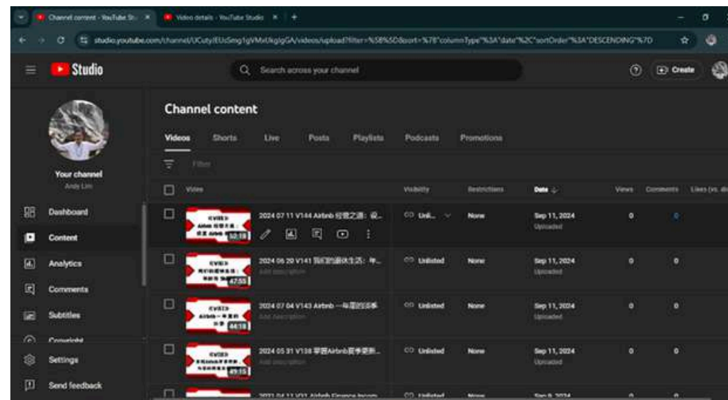
Upload video
