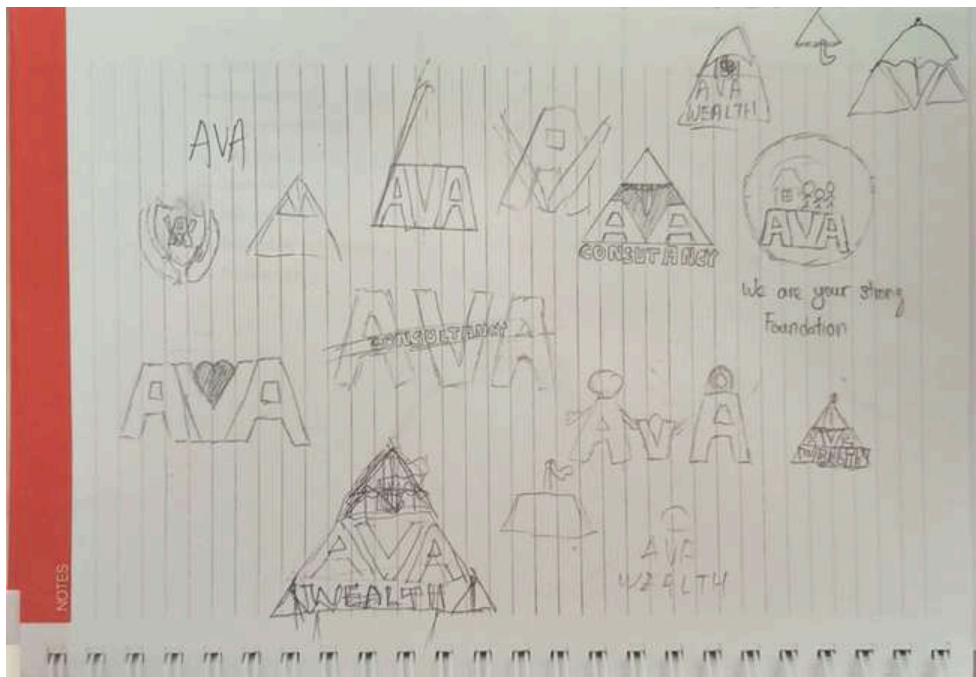
Design Logo
