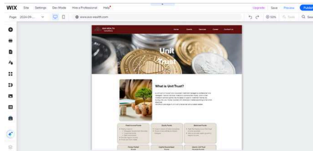
Design Website
